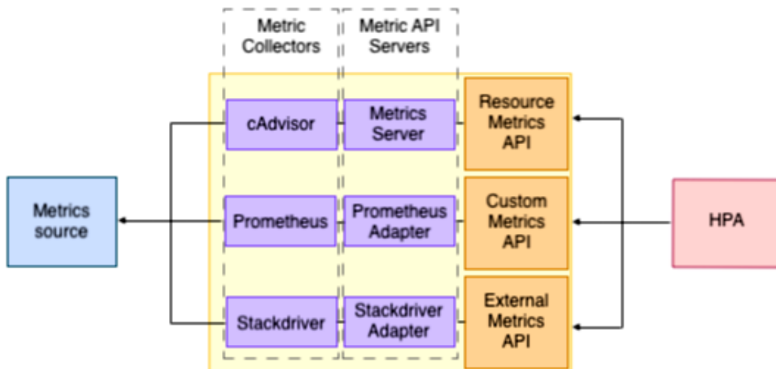
Figure 4. Diagram of metrics registry components 655
