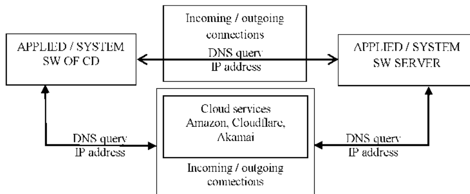
Fig. 6. Diagram of software access to the Internet
