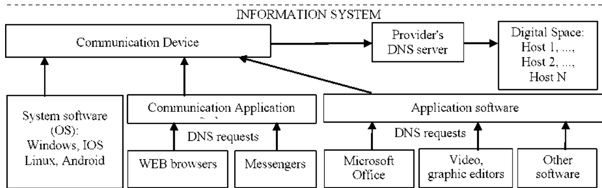
Fig. 2. Interaction of IS modules with digital space
