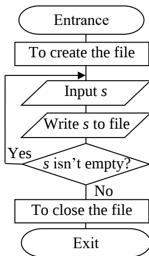
Flowchart of function create_file()
